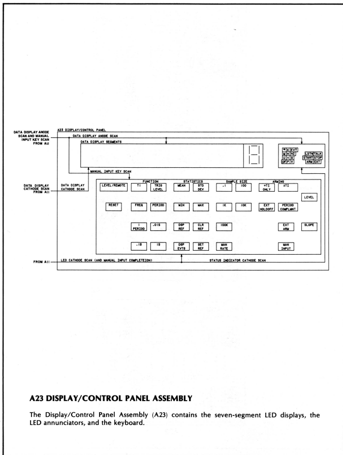
Part of Figure 8-36. A23 Front Panel Display/Control Assembly
