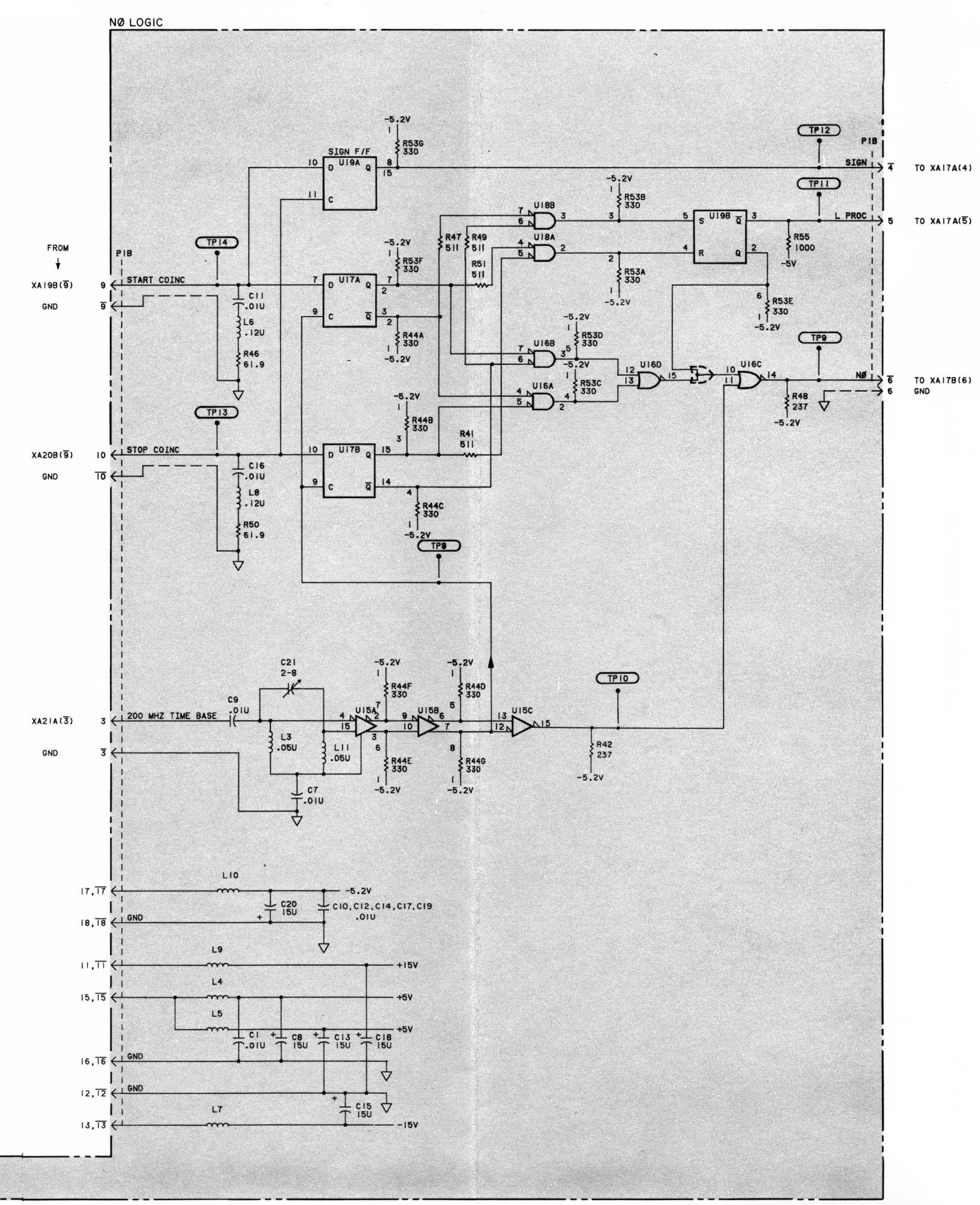
Figure 8-32. A18 DAC/N0 Logic Assembly
