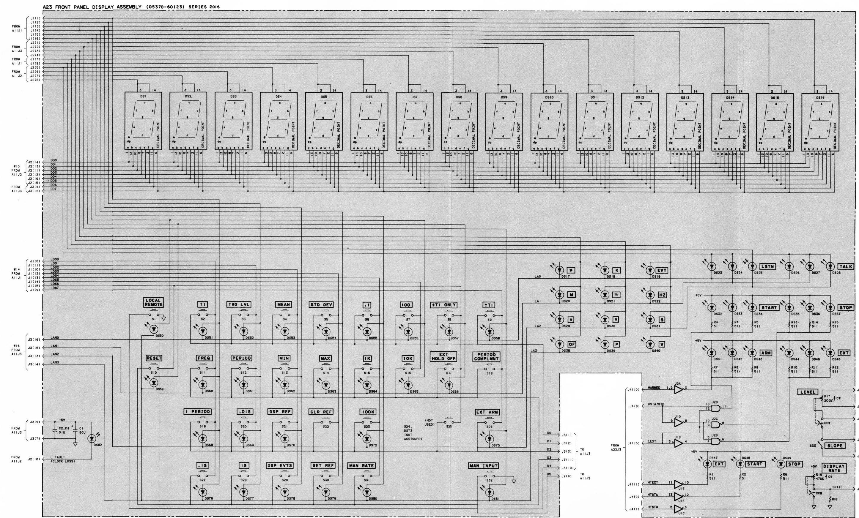
Figure 8-36. A23 Front Panel Display Assembly
