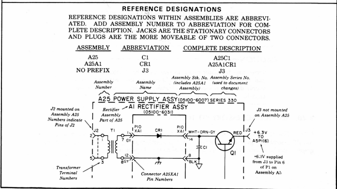
Figure 8-1. Schematic Diagrams Notes
