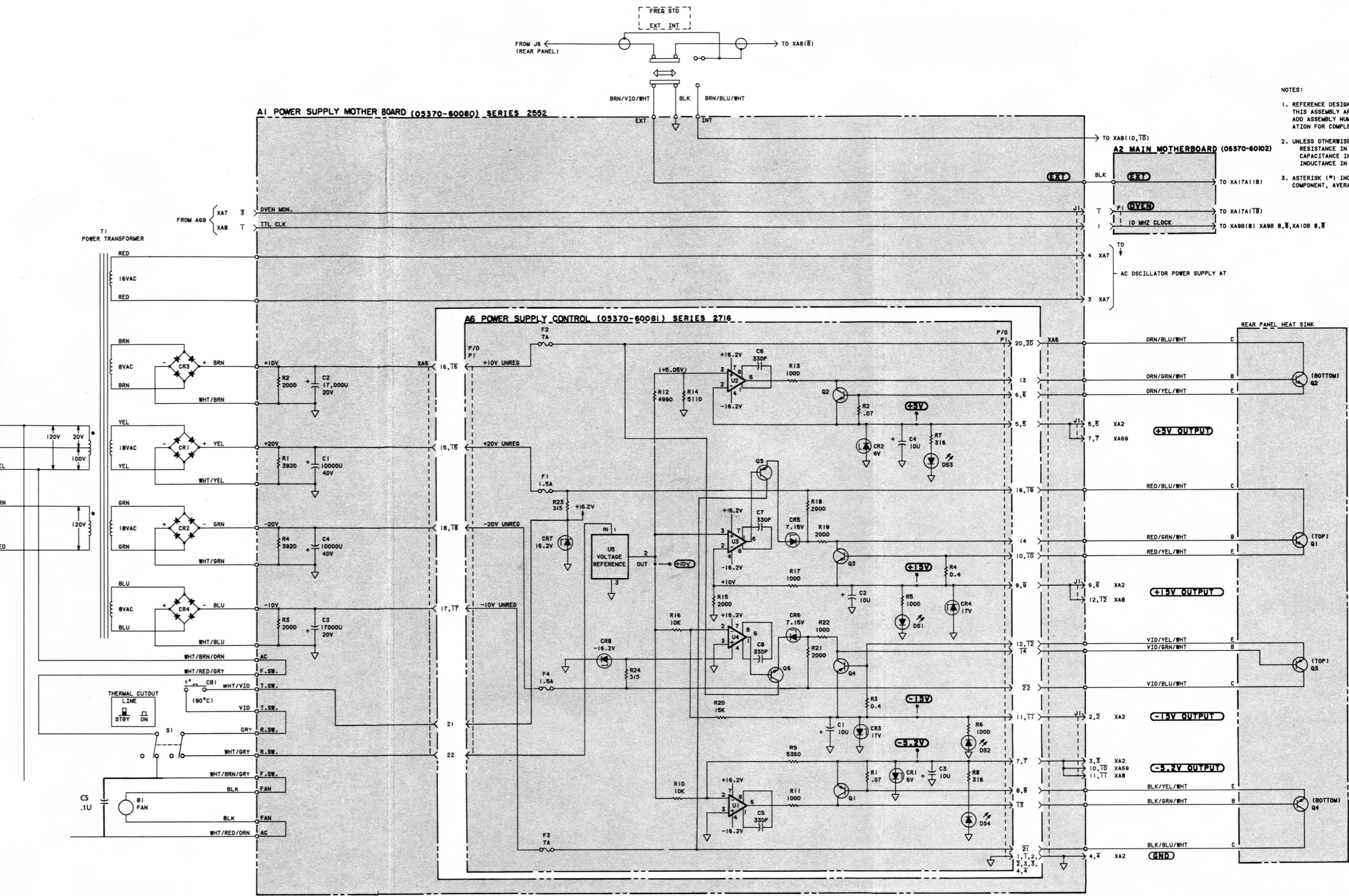
Figure 8-22. A1 Power Supply/Motherboard Assembly, A6 Power Supply Control Assembly, A24 Line Module Assembly
