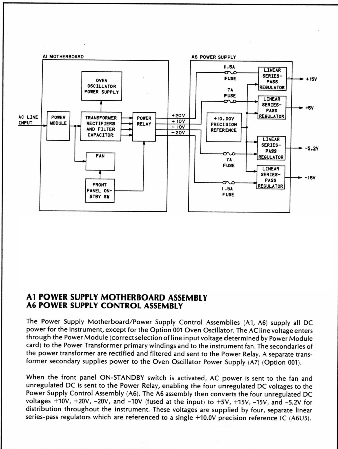
Figure 7-2. A1 Power Supply Motherboard, A6 Power Supply Control Assembly
