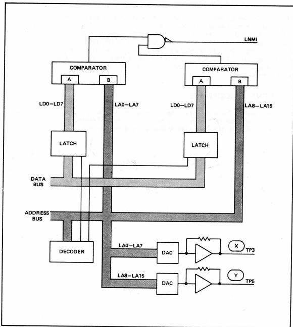
Figure 8-4. 05370-60014 Block Diagram
