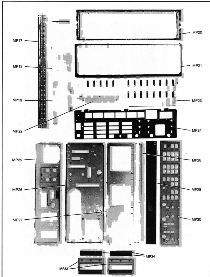
Figure 6-1. Mechanical Parts ( Continued)
