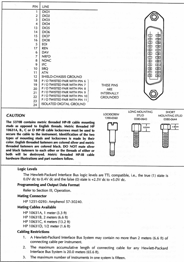
Figure 2-3. Hewlett-Packard Interface Bus Connection
